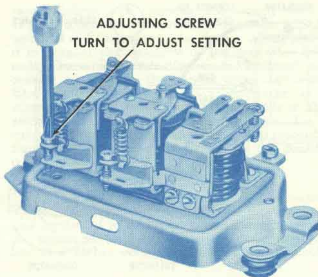
Figure 6—Adjusting voltage regulator setting.
